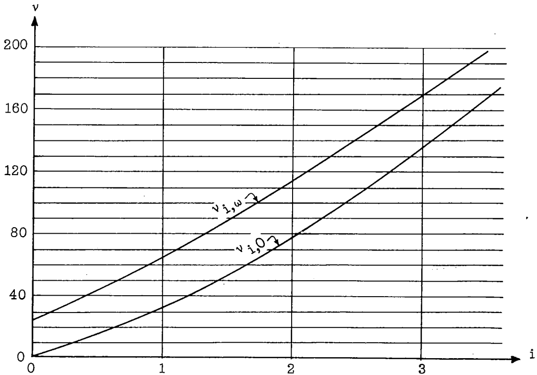
Figure 6.- Natural frequencies of the N.C.2001 blade.
