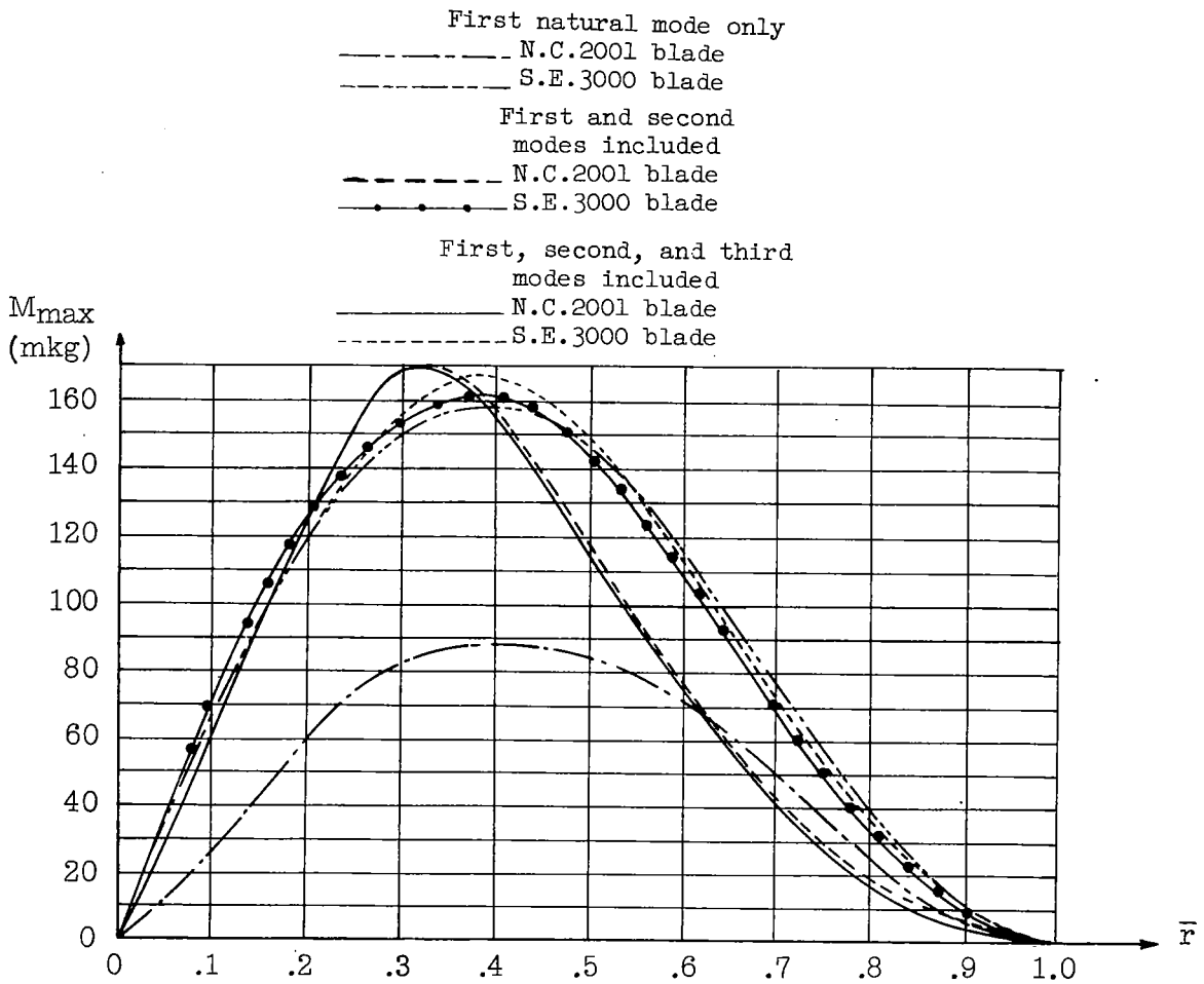
Figure 14.- Maximum bending moments.
