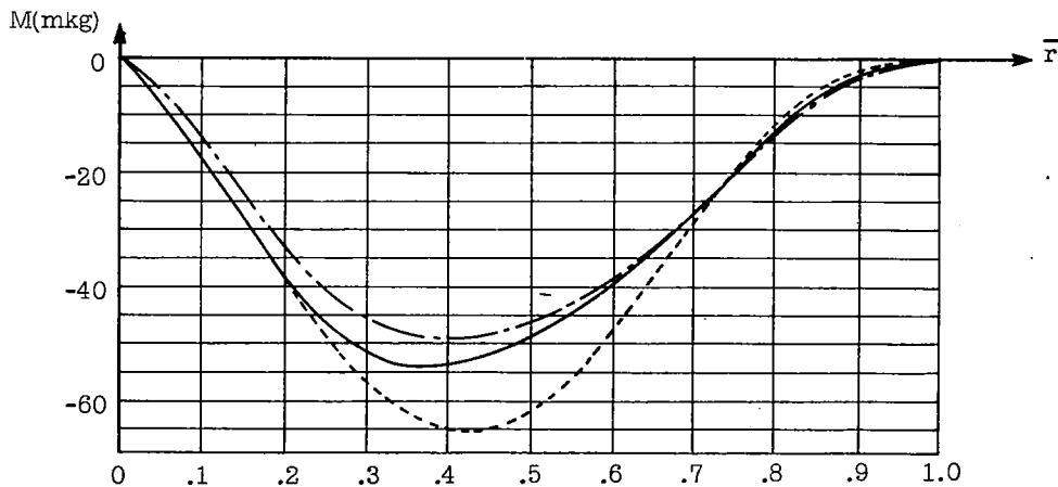
Figure 9.- N.C.2001 blade - blade bending moments for \psi = 0 .
