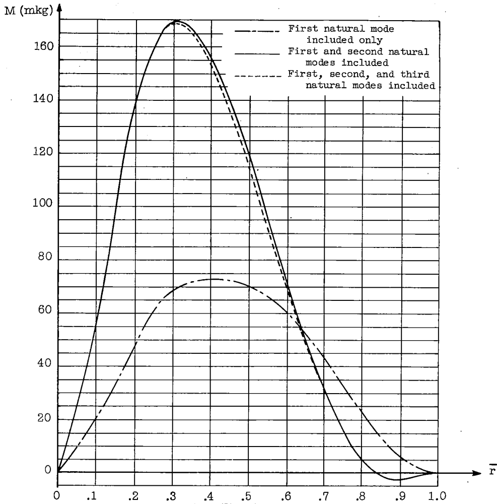
Figure 9.- N.C.2001 blade - blade bending moments for \psi = 0 .
