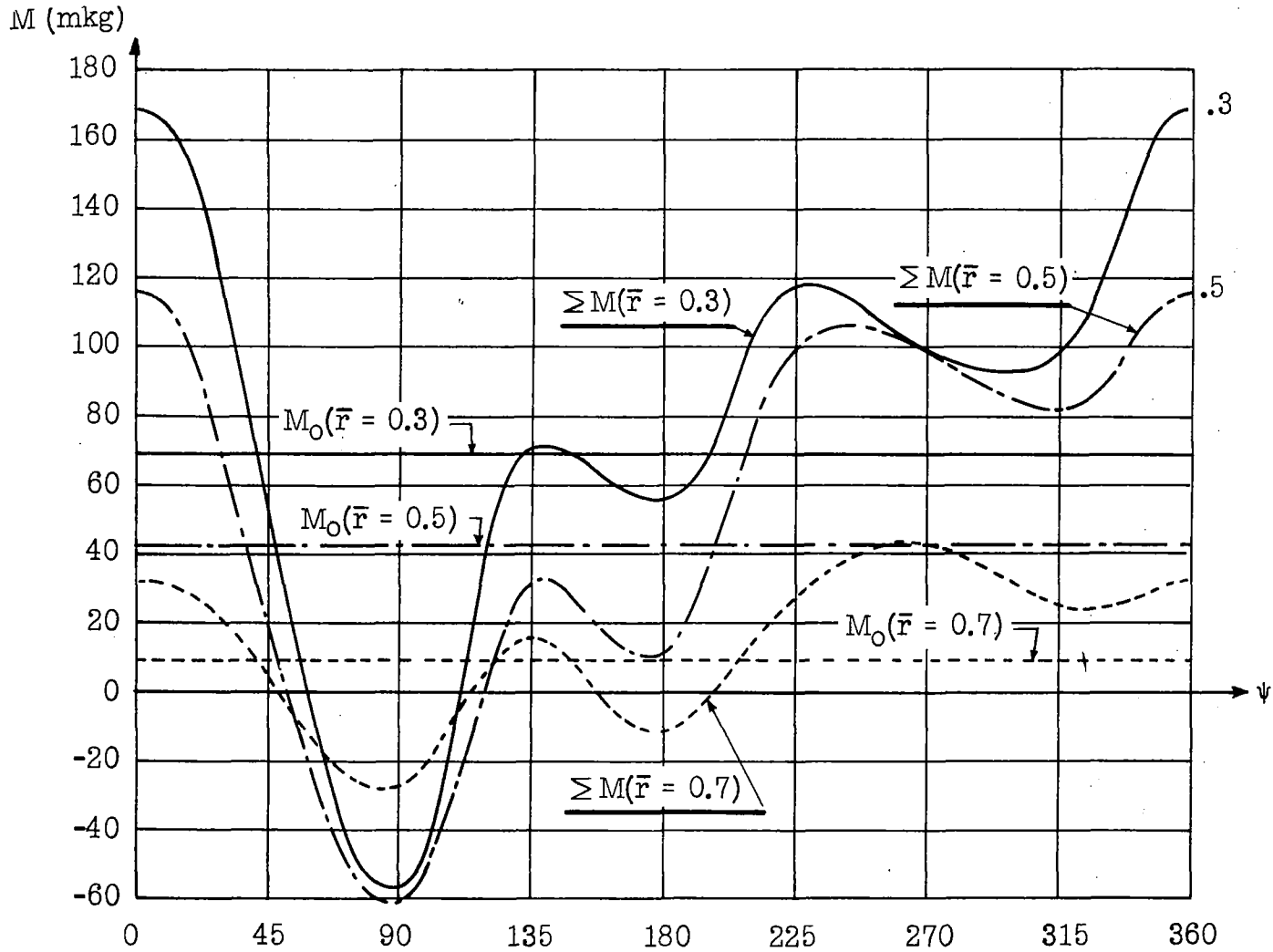
Figure 13.- N.C.2001 blade - blade bending moments plotted against \psi .
