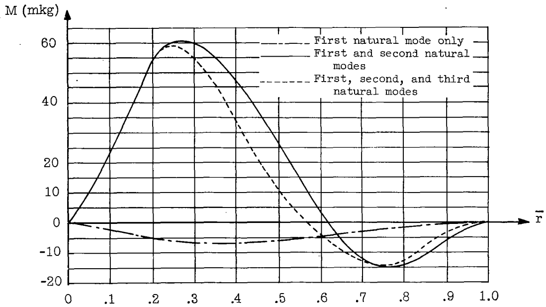
Figure 11.- N.C.2001 blade - blade bending moments for \psi = 180^\circ .
