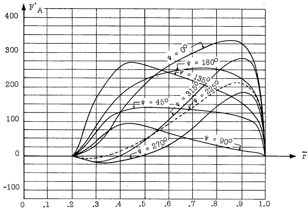
Figure 7.- N.C.2001 blade - distribution of aerodynamic forces F'_A on the rigid blade.
