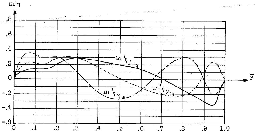
Figure 5.- N.C.2001 blade - natural distributions m'v^2\eta = \frac{d^2}{dx^2} \left( EI \frac{d^2\eta}{dx^2} \right) for v = 1 .
